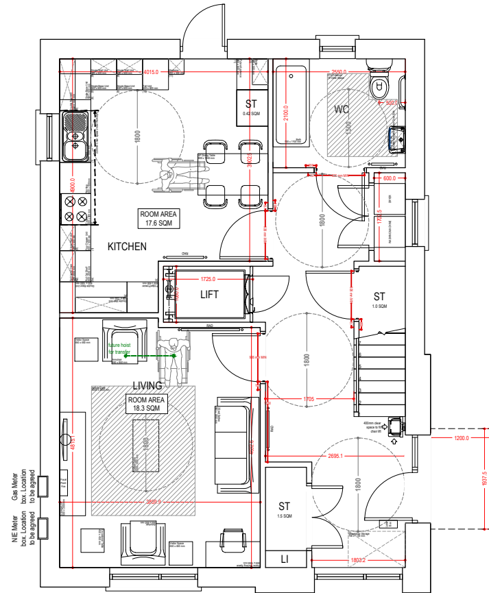
GROUND FLOOR W5P3B HTE 130 SQM
