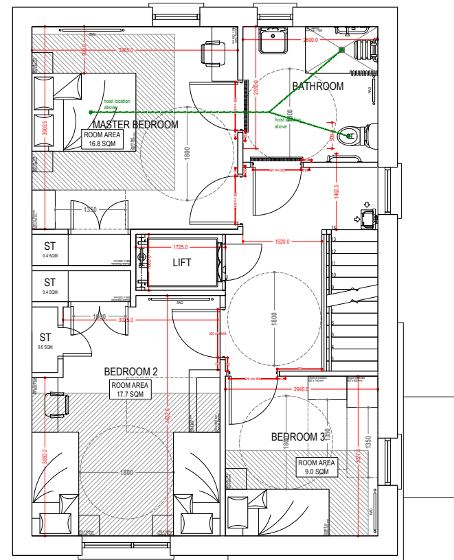
FIRST FLOOR W5P3B HTE 130 SQM
