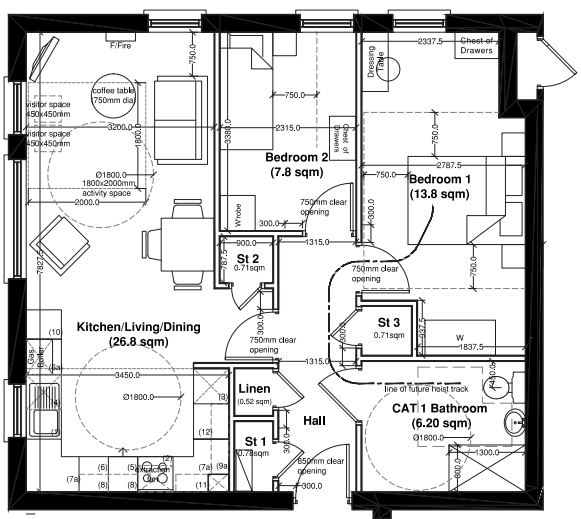
Block A Upper Floor Apartment
