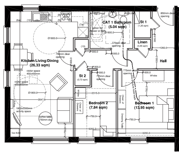
Block B Upper Floor Apartment
